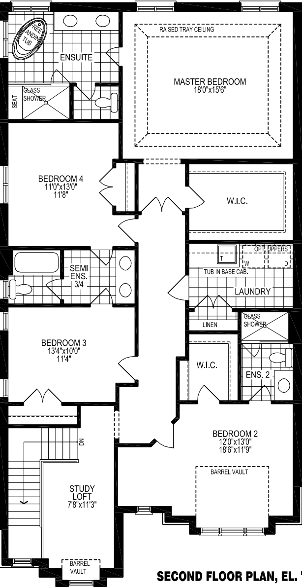
SECOND FLOOR PLAN, EL. 'A'
