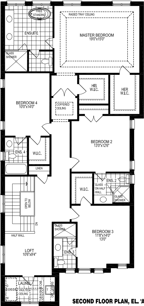
SECOND FLOOR PLAN, EL. 'A'
