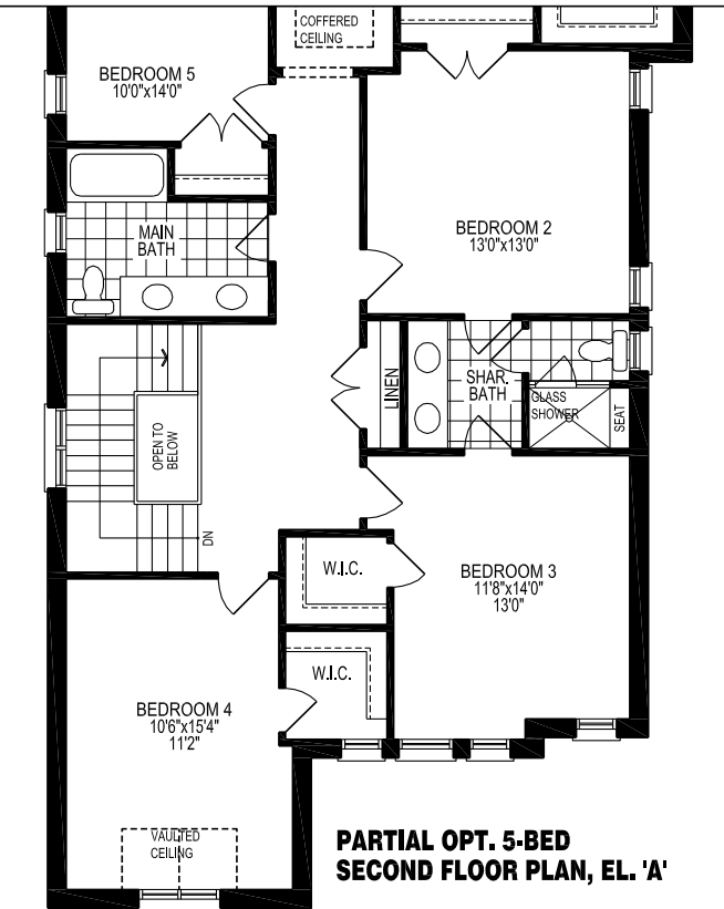
SECOND FLOOR PLAN, EL. 'A'
