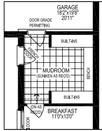
PART. ALT. GROUND FLOOR PLAN WITHOUT SECONDARY STAIR
