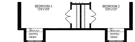
PARTIAL SECOND FLOOR PLAN, EL. 'B'
