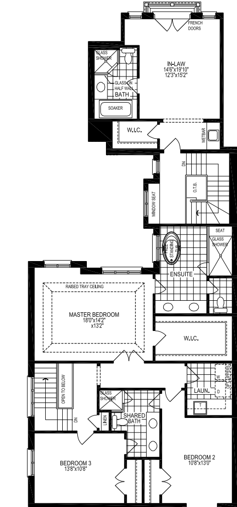
SECOND FLOOR PLAN, EL. 'A'
