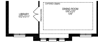
PARTIAL MAIN FLOOR PLAN, EL. 'B'
