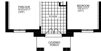
PARTIAL LOWER LEVEL PLAN, EL. 'B'
