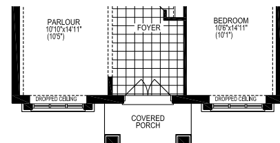
PARTIAL LOWER LEVEL PLAN, EL. 'C'
