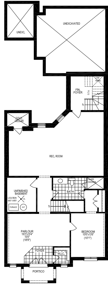
LOWER LEVEL PLAN, EL. 'A'
