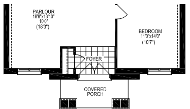
PARTIAL LOWER LEVEL PLAN, EL. 'B'
