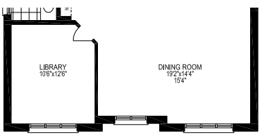
PARTIAL MAIN FLOOR PLAN, EL. 'C'
