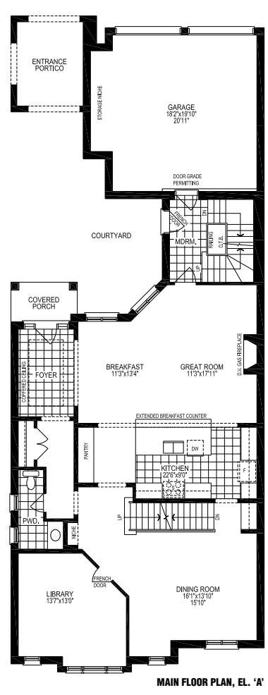
MAIN FLOOR PLAN, EL. 'A'
