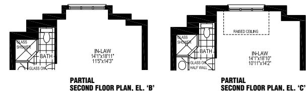
PARTIAL SECOND FLOOR PLAN, EL. 'B'
