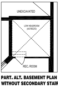
PART, ALT. BASEMENT PLAN WITHOUT SECONDARY STAIR
