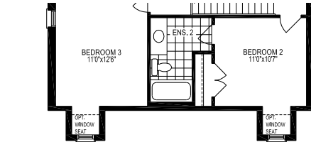
PARTIAL SECOND FLOOR PLAN, EL. 'B'
