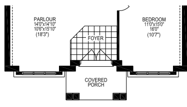
PARTIAL LOWER LEVEL PLAN, EL. 'C'
