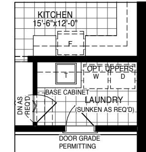
GROUND FLR. PLAN W/ LAUND. FOR OP. 5-BEDRM PLAN
