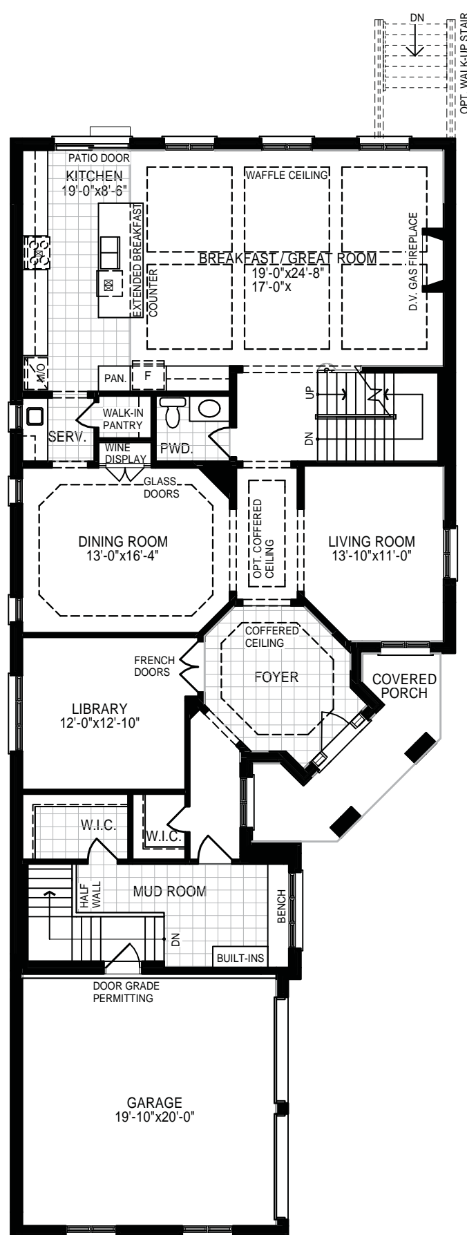
ELEV. A MAIN LEVEL
